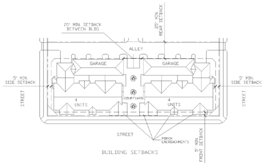
BUILDING SETBACKS
