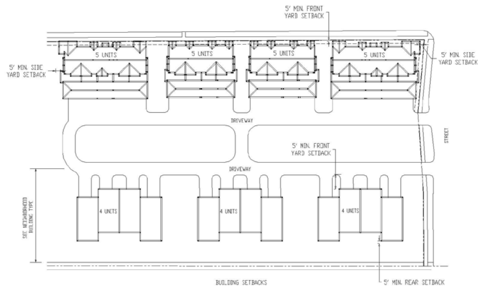
BUILDING SETBACKS
